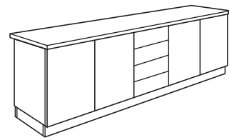
606 CBB (Chipboard Top) Low Cabinet 2010W. x 456D. x 710H. mm. 79¼"W. x 18"D. x 28"H. inch.
