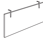
VN 2190-WFP Wooden Front Panel with Bracket 930W. x 400D. x 18H. mm. 36¾"W. x 15¾"D. x ¾"H. inch.
